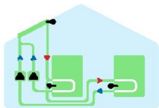
solar + storage tank loading circulating pump
